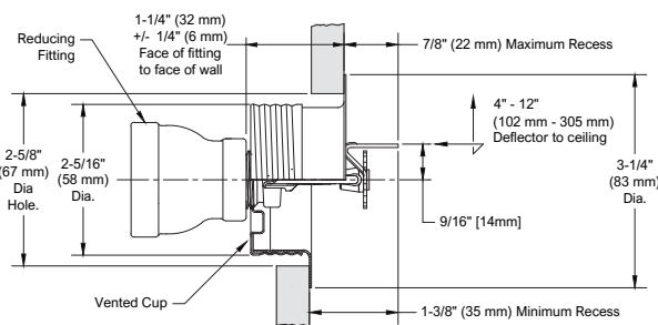
Model F1FR Horizontal Sidewall Sprinkler with Model FP Recessed Escutcheon 1/2" (13mm) Nominal Adjustment
