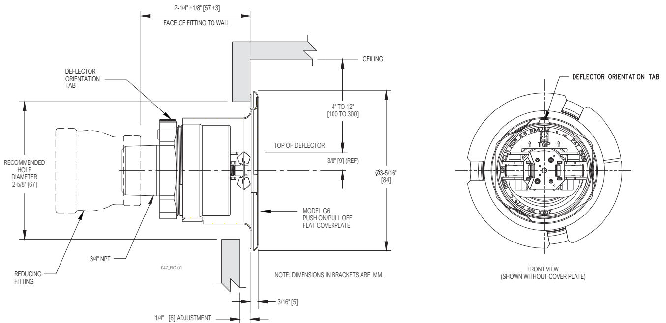
Model G6-80 Concealed Sidewall Sprinkler Components and Dimensions
