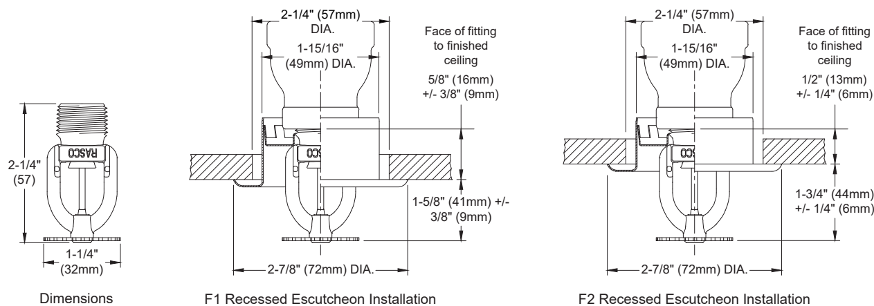
Model F1Res49 LL Residential Pendant Sprinkler Hydraulic Design Criteria
