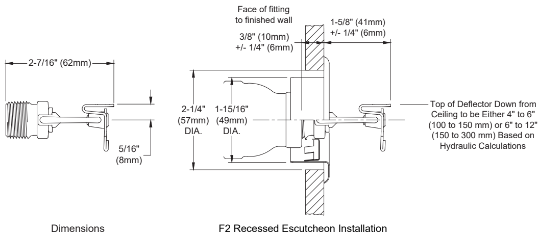
Model F1Res44 LL Horizontal Sidewall Sprinkler Hydraulic Design Criteria
