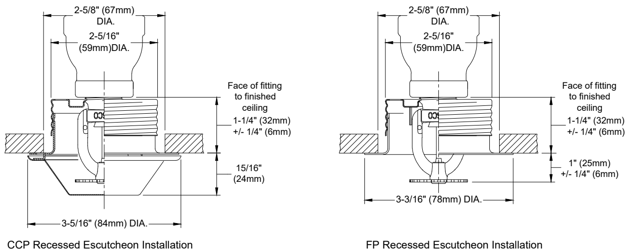
Model F1Res58 LL CCP and FP Recessed Pendent Sprinkler Installation Dimensions Figure 6
