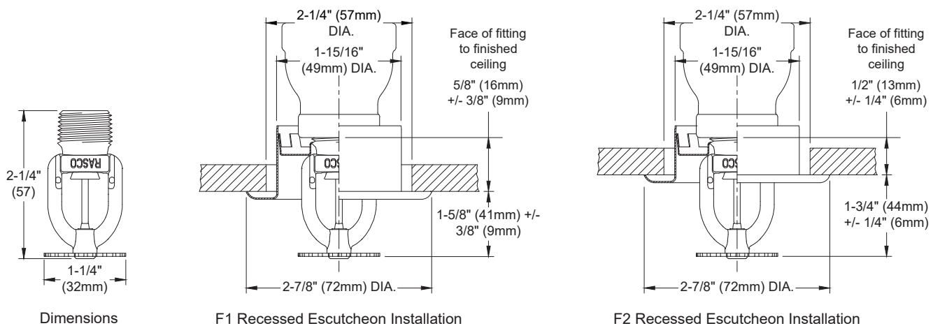
Model F1Res58 LL Residential Pendent Sprinkler Components and Installation Dimensions Figure 3
