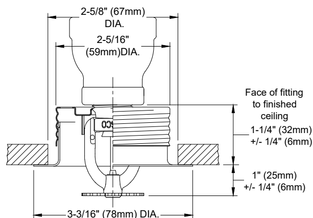
Model F1Res49 LL CCP & FP Recessed Pendent Sprinkler Installation Dimensions
