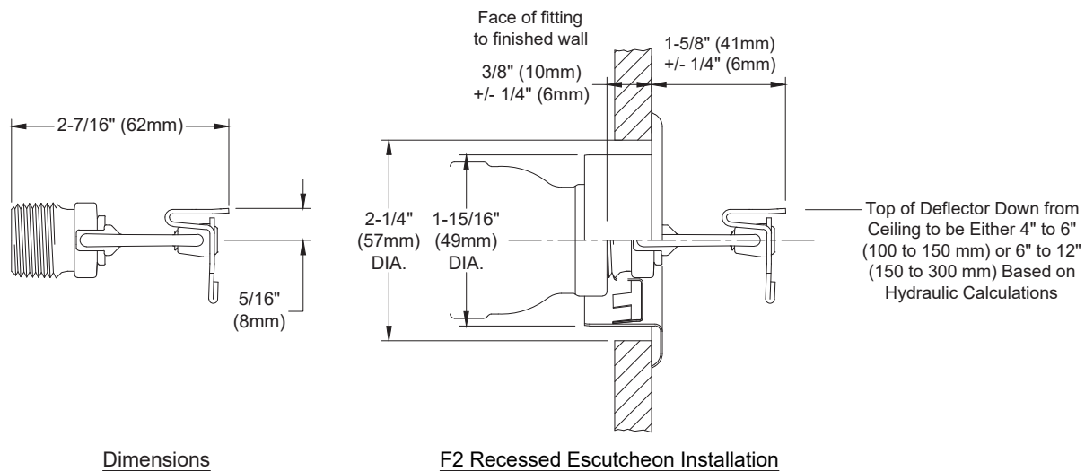
Model F1Res58 LL Residential Horizontal Sidewall Sprinkler Installation Dimensions
