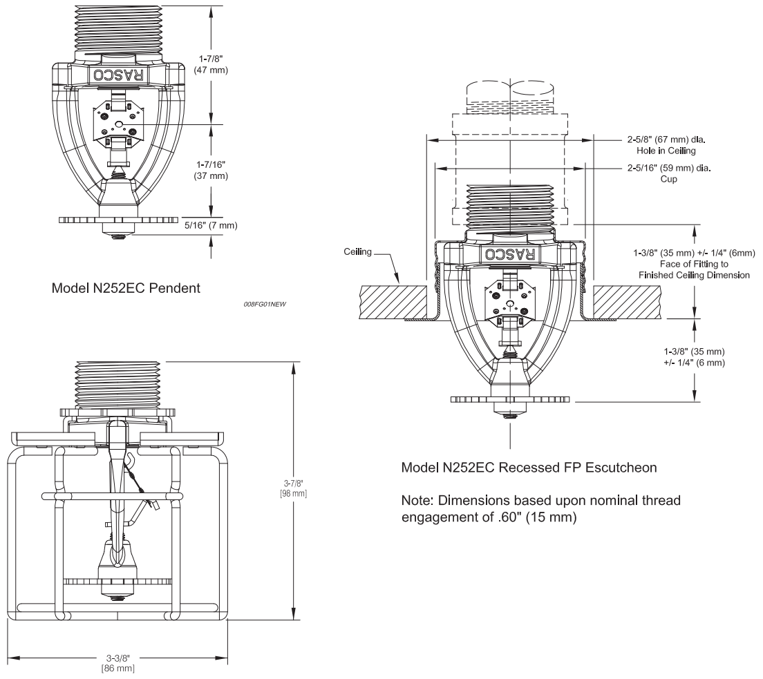
Model N252EC Pendent with Model 25 Guard (Shown rotated 90 degrees; FM Approved for use as an in-rack sprinkler)
