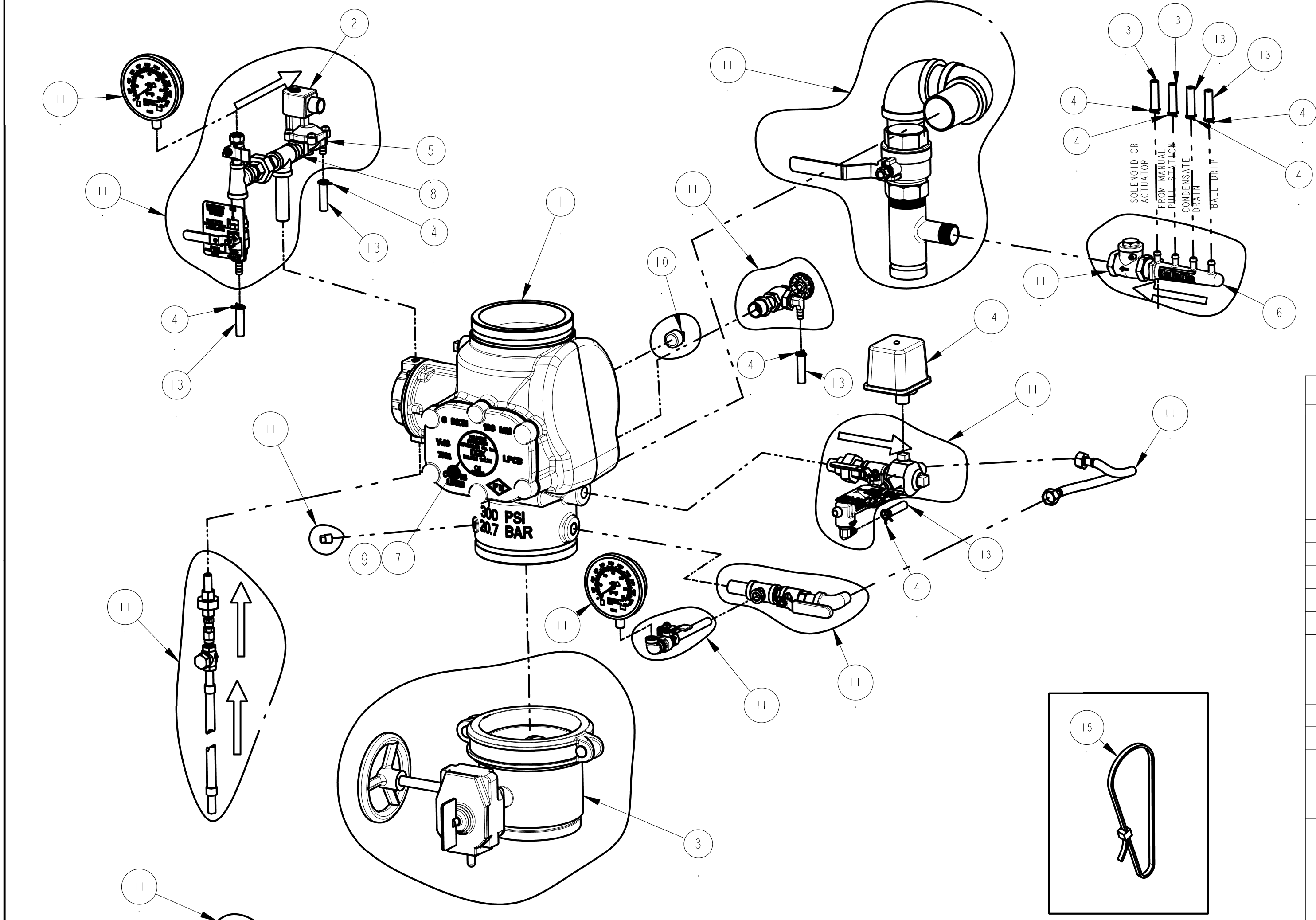
MODEL DDX 4", 6" & 8" DELUGE ELECTRIC ACTUATION CA-154 P/N 89241118
