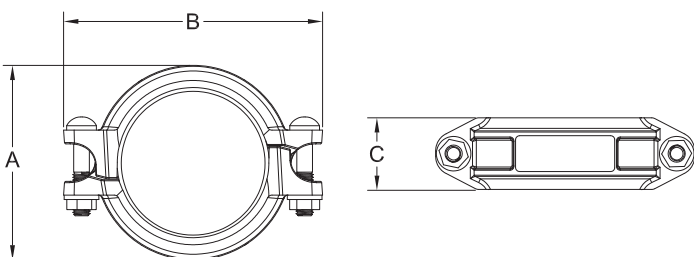
RGD1 Angled Pad Coupling Dimensions Figure 1
